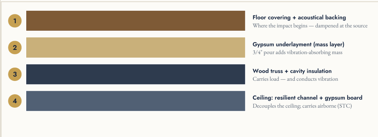
Figure (A3). The four layers of a wood-framed floor-ceiling assembly. The IIC and HIIC ratings reflect the combined performance of all four layers.
