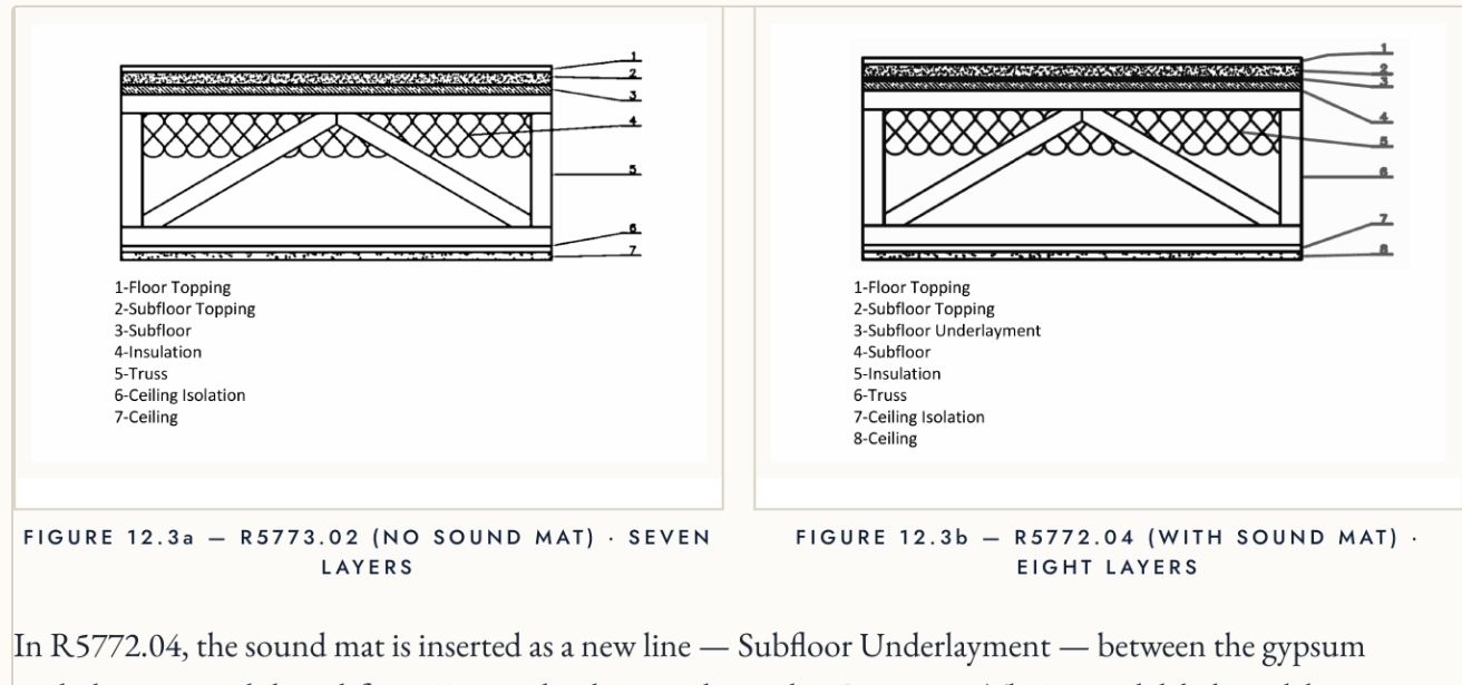
FIGURE 12.3 Left: R5773.02 (no sound mat), seven layers. Right: R5772.04 (with sound mat), eight layers. In R5772.04 the sound mat is inserted as a new line — Subfloor Underlayment — between the gypsum underlayment and the subfloor. Every other layer is identical.
